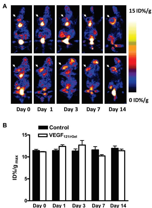
Figure 2. (A) Representative decay-corrected whole-body coronal microPET images of mice bearing MDA-MB-435 breast cancer at 1 h after intravenous injection of 18 F-FDG (1.85 MBq/mouse) on days 0, 1, 3, 7, and 14 after the treatment was initiated. The tumors are indicated by arrows. Upper panel: control. Lower panel: VEGF 121 /rGel treatment. (B) Tumor uptake of 18 F-FDG quantified by ROI analysis.
