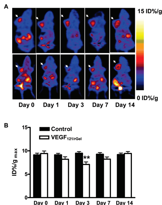
Figure 3. (A) Representative decay-corrected whole-body coronal microPET images of mice bearing MDA-MB-435 breast cancer at 1.5 h after intravenous injection of 18 F-FLT (1.85 MBq/mouse) on days 0, 1, 3, 7, and 14 after the treatment was initiated. The tumors are indicated by arrows. Decreased uptake of 18 F-FLT was observed on day 1 and day 3 but resumed to baseline level on day 7. Upper panel: control. Lower panel: VEGF 121 /rGel treatment. (B) Quantitative microPET region of interest analysis of tumor uptake for 18 F-FLT. (** p < 0.01 ).
