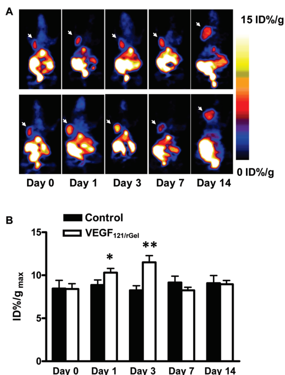
Figure 4. (A) Representative decay-corrected whole-body coronal microPET images of mice bearing MDA-MB-435 breast cancer at 2.5 h after intravenous injection of ^{18}\text{F} -FMISO (1.11 MBq/mouse) on days 0, 1, 3, 7, and 14 after the treatment was initiated. The tumors are indicated by arrows. Increased tumor uptake of ^{18}\text{F} -FMISO was observed on day 1 and day 3 but was restored to the baseline level on day 7. Upper panel: control. Lower panel: VEGF 121 /rGel treatment. (B) Quantitative microPET region of interest analysis of tumor uptake for ^{18}\text{F} -FMISO. (* p < 0.05 , ** p < 0.01 ).
